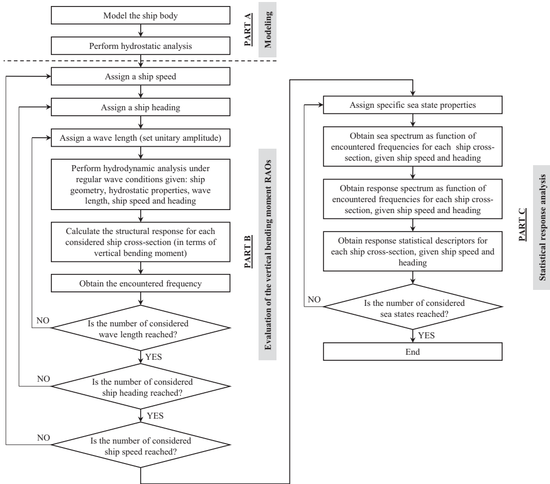
Figure 5.1 Flowchart of the procedure for the probabilistic evaluation of the ship load due to waves for generic operational conditions.
