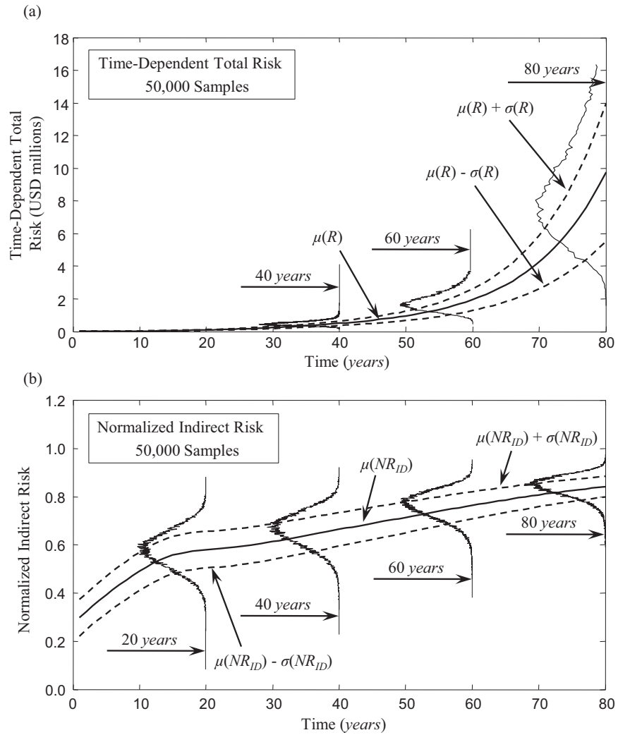
Figure 2.11 Profiles of (a) mean ( \mu ) and mean plus ( \mu + \sigma ) and minus ( \mu - \sigma ) one standard deviation of the total time-dependent risk, and (b) normalized indirect risk index ( NR_{ID} ).
