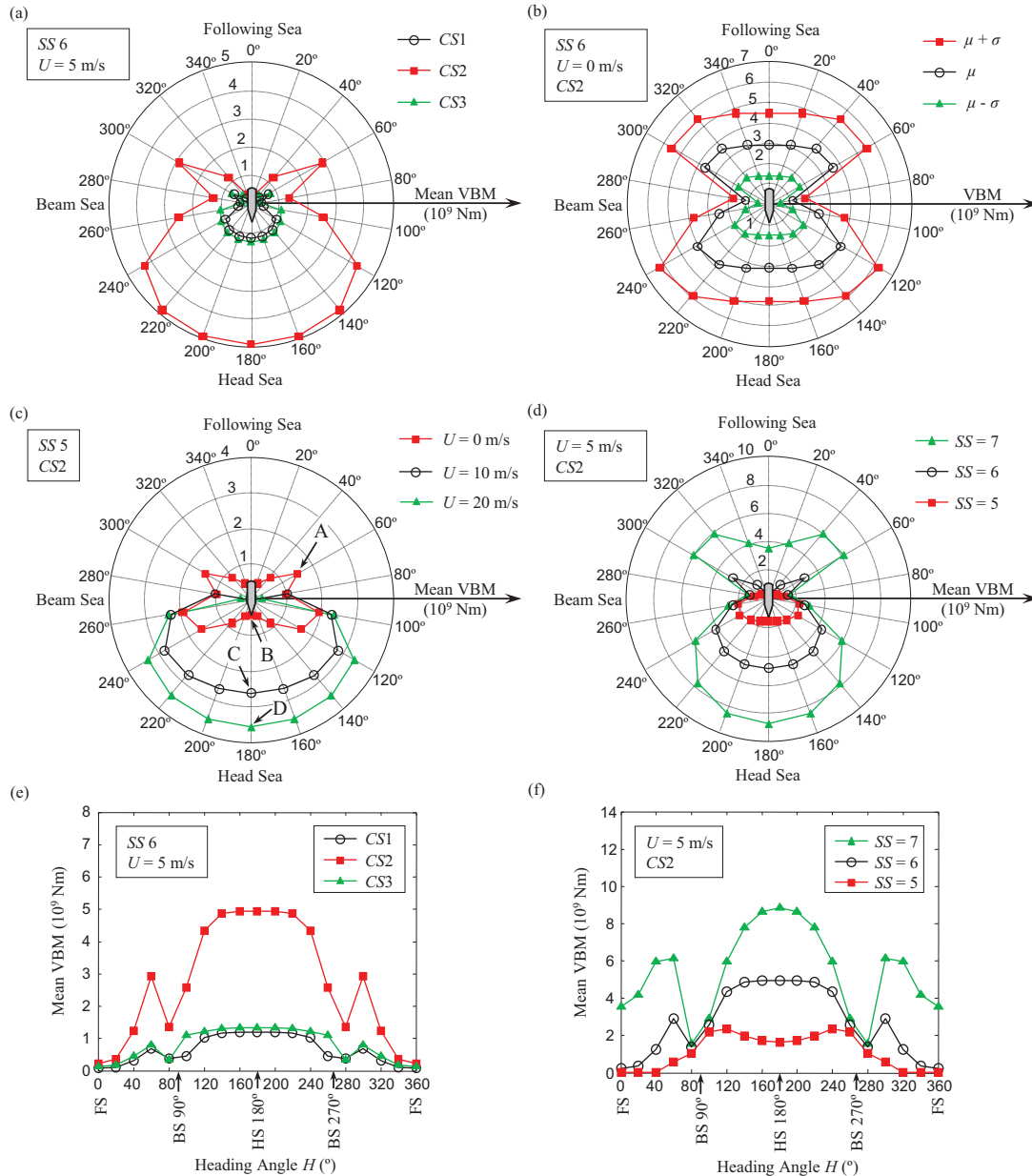
Figure 5.7 Polar representation of the VBM. (a) Profiles of mean VBM for different cross-sections, (b) profiles of mean and mean plus and minus one standard deviation of the VBM, (c) profiles of mean VBM for CS2 and sea state 5 by varying ship speed, and (d) profiles of mean VBM for CS2 and ship speed of 5 m/s by varying sea state. Plots of mean VBM (e) for different cross-sections and (f) for CS2 by varying sea state.
